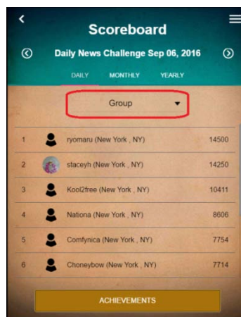
Leaderboard/Results
