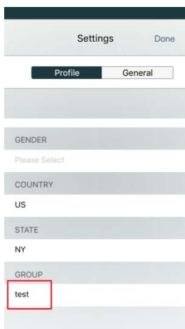
Mobile App
